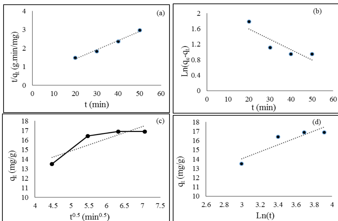
Figure 7. plot of a) pseudo-second order b) pseudo- first order c) Intraparticle diffusion d) Elovich in MB-modified gypsum system
